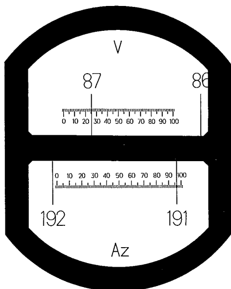
Figure 8 Circle readings (400 \times ): Vertical (V) 87.255 ^{\circ} ; Horizontal (Az) 191.965 ^{\circ} (Horizontal circle appears yellow; vertical, white)
